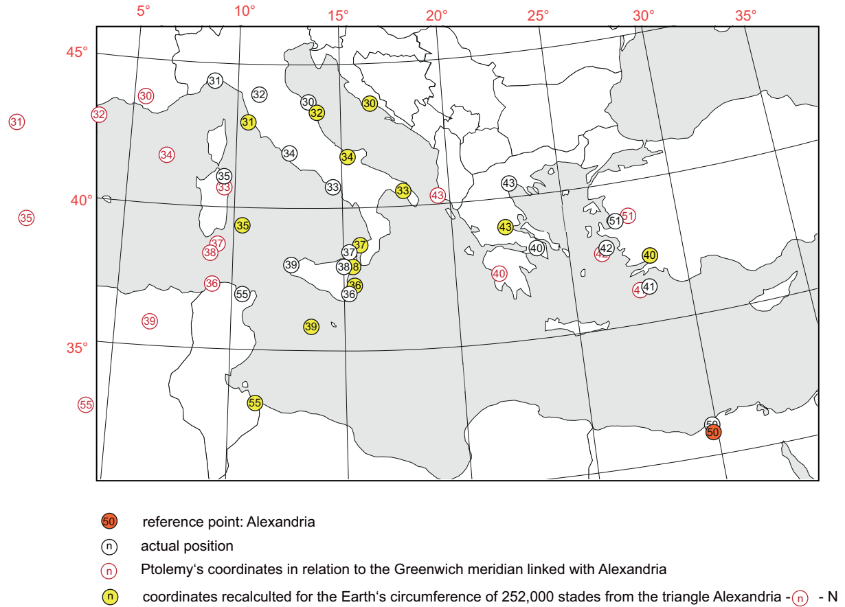
Figure 6: Recalculation of some prominent locations in the eastern Mediterranean for the circumference of the Earth equal to 252,000 stades. The reference point for this recalculation is Alexandria.
