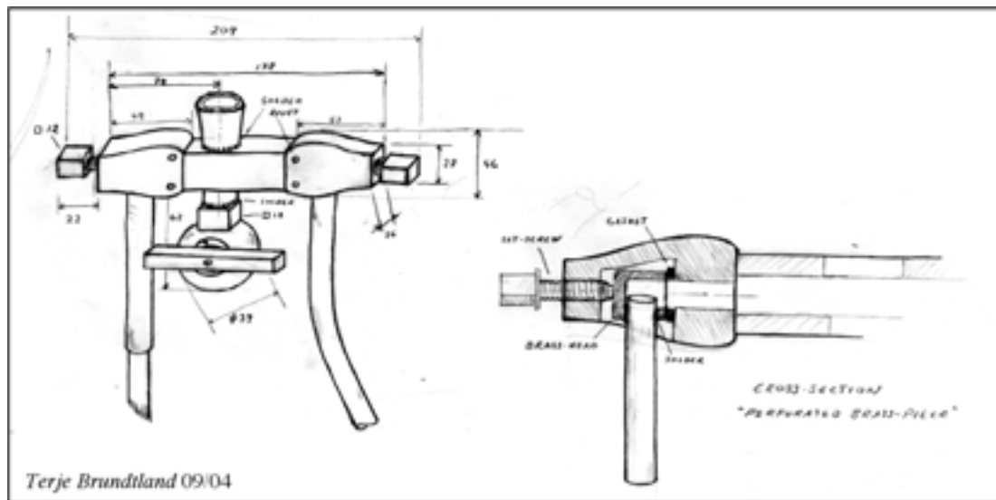
Figure 3: A perforated brass-piece.
