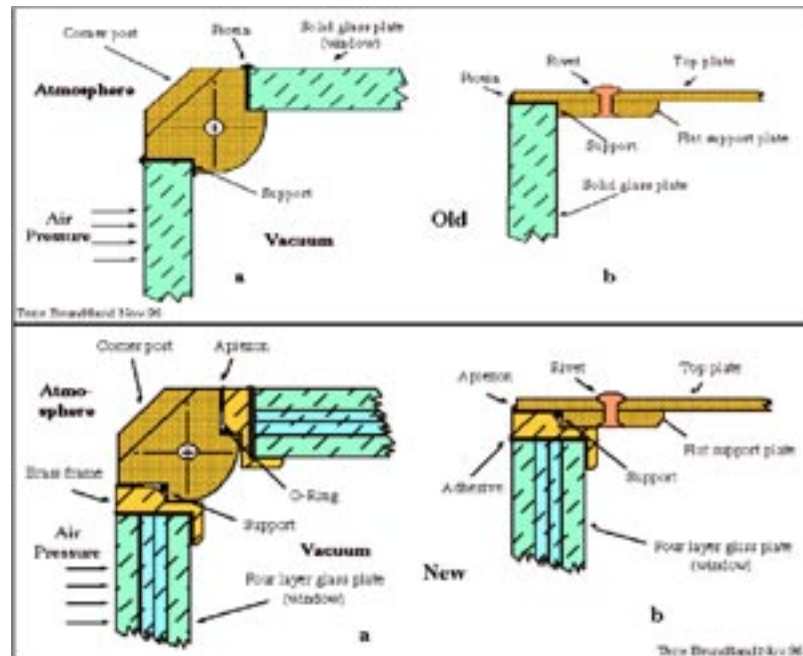
Figure 7: Old and new windows. a: top view. b: side view.
