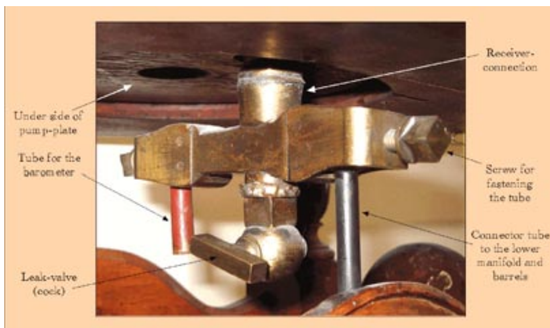
Figure 4: Upper manifold. Photo: Terje Brundtland.
