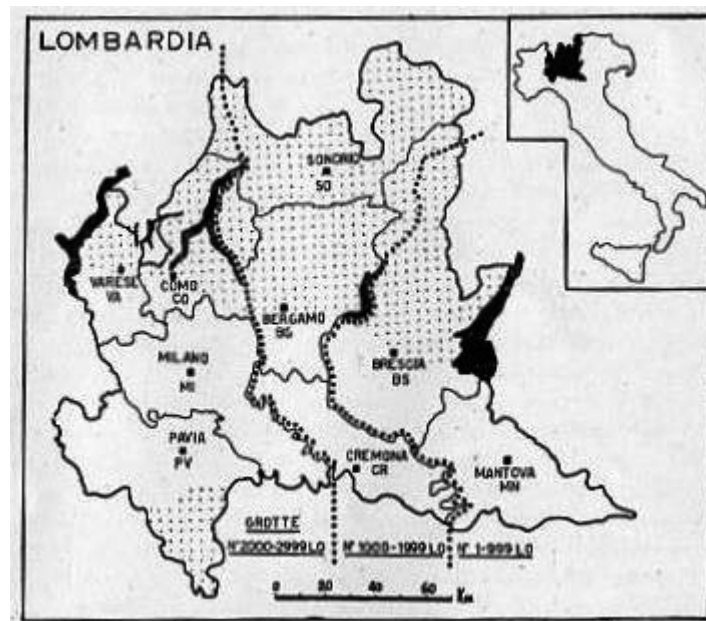
Figure 4: Map of Lombardy for the usage of the national speleologic register. The division into three areas assumes an unusual east to west direction, probably due to the intensity of research in East Lombardy at the same period that the register was established.
