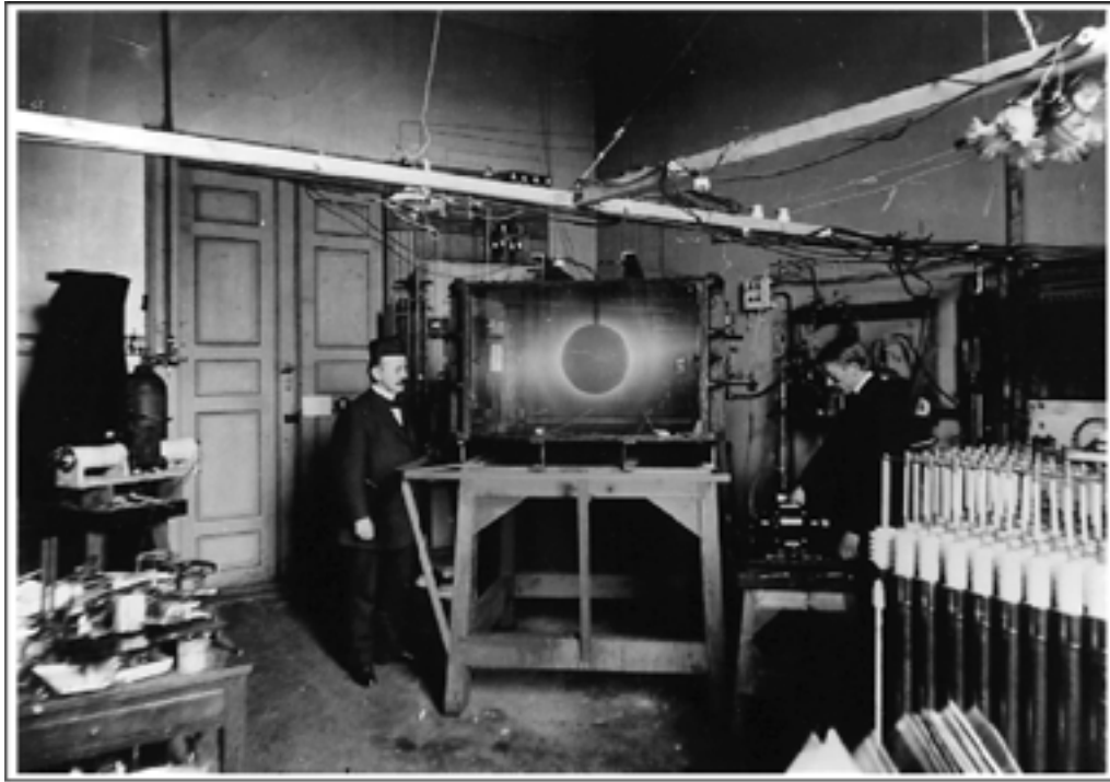
Figure 6: Professor Birkeland's Terrella Experiment. Christiania (Oslo), 1913.
