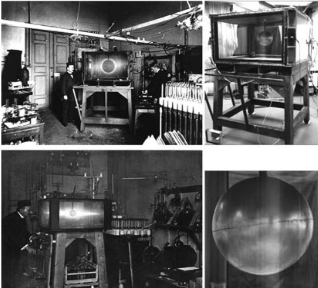
Figure 5: Kristian Birkeland's "Terrella" in Tromsø. On the left: Birkeland at work in his laboratory in 1913. On the right: the "Terrella" after its restoration in 1995.
