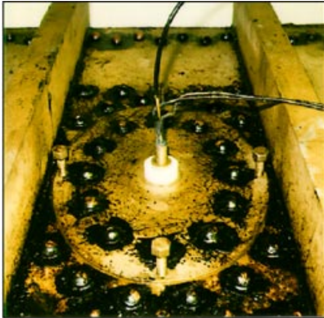
Figure 8: Tar on rivets and along fissures. Photo: Terje Brundtland.
