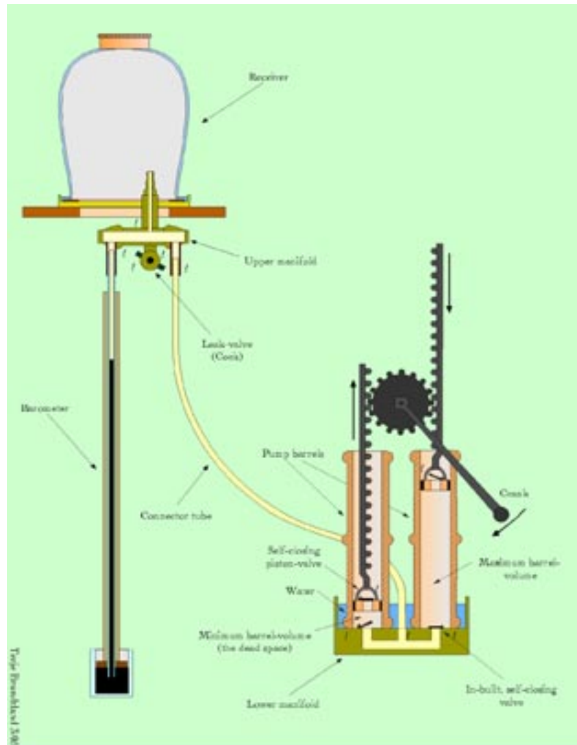
Figure 5: Functional diagram.
