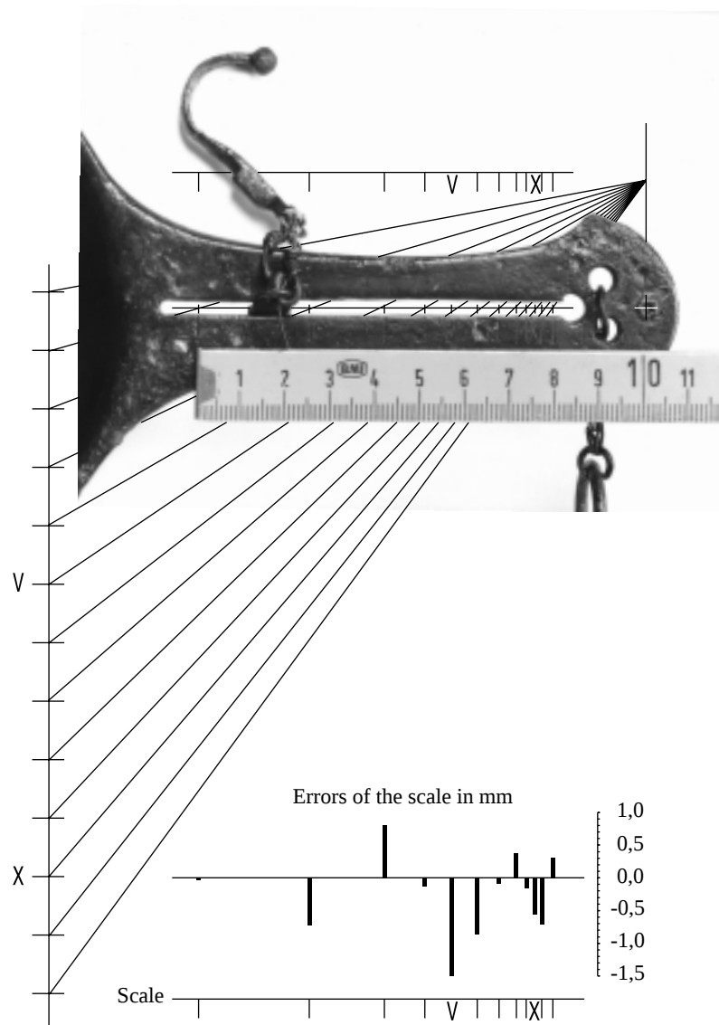
Figure 3. SCALE OF THE “CASSEROLE BISMAR”
