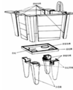
Figure 11: The square ding from the storage pit in Zhengzhou (upper H1:3) and its casting joint structure (left: from The Bronzes in the Storage Pit in Zhengzhou , plate 5; right: from The Bronzes in the Storage Pit in Zhengzhou , p.11, fig. 3).
